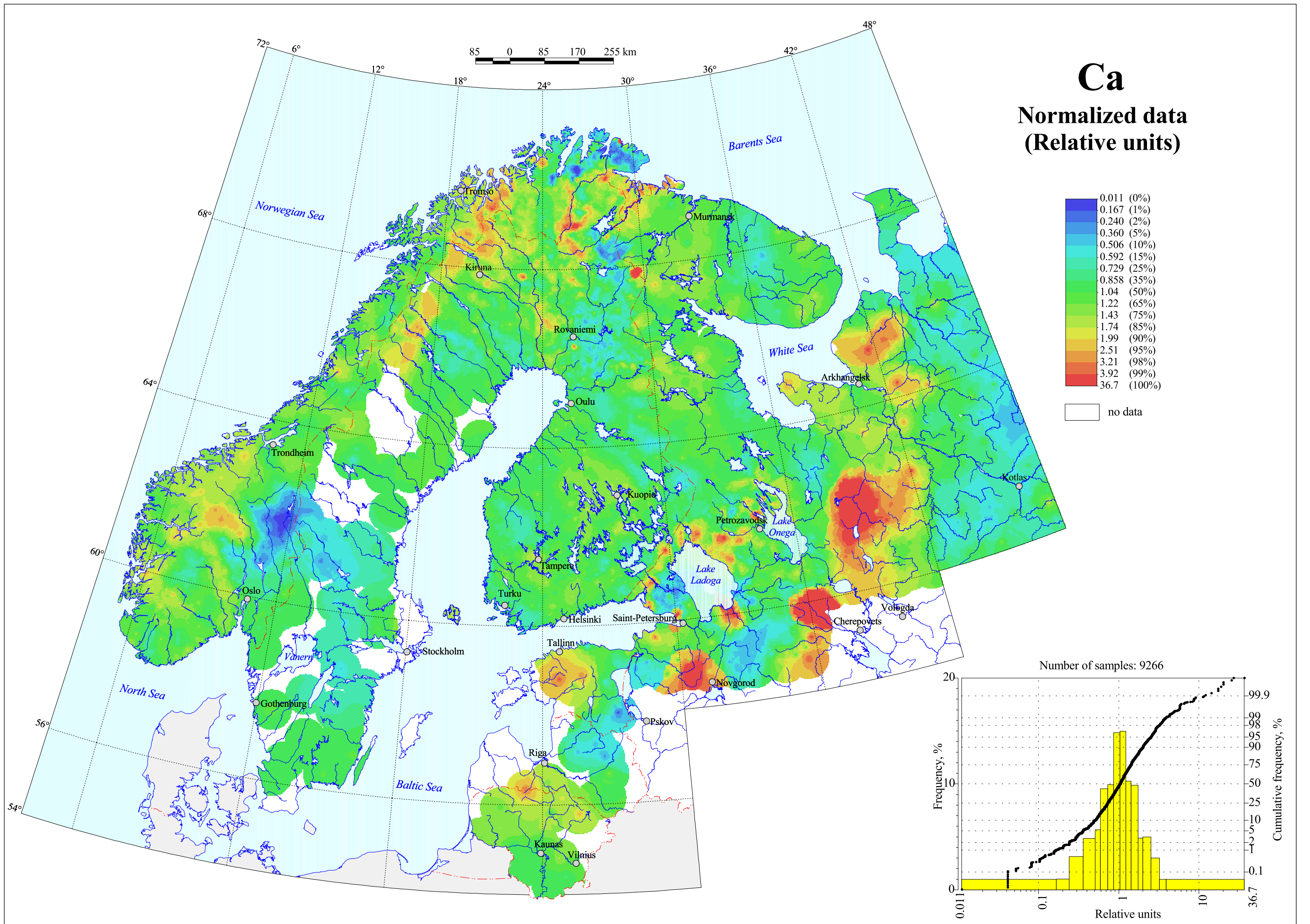
Calcium in Stream Sediment
